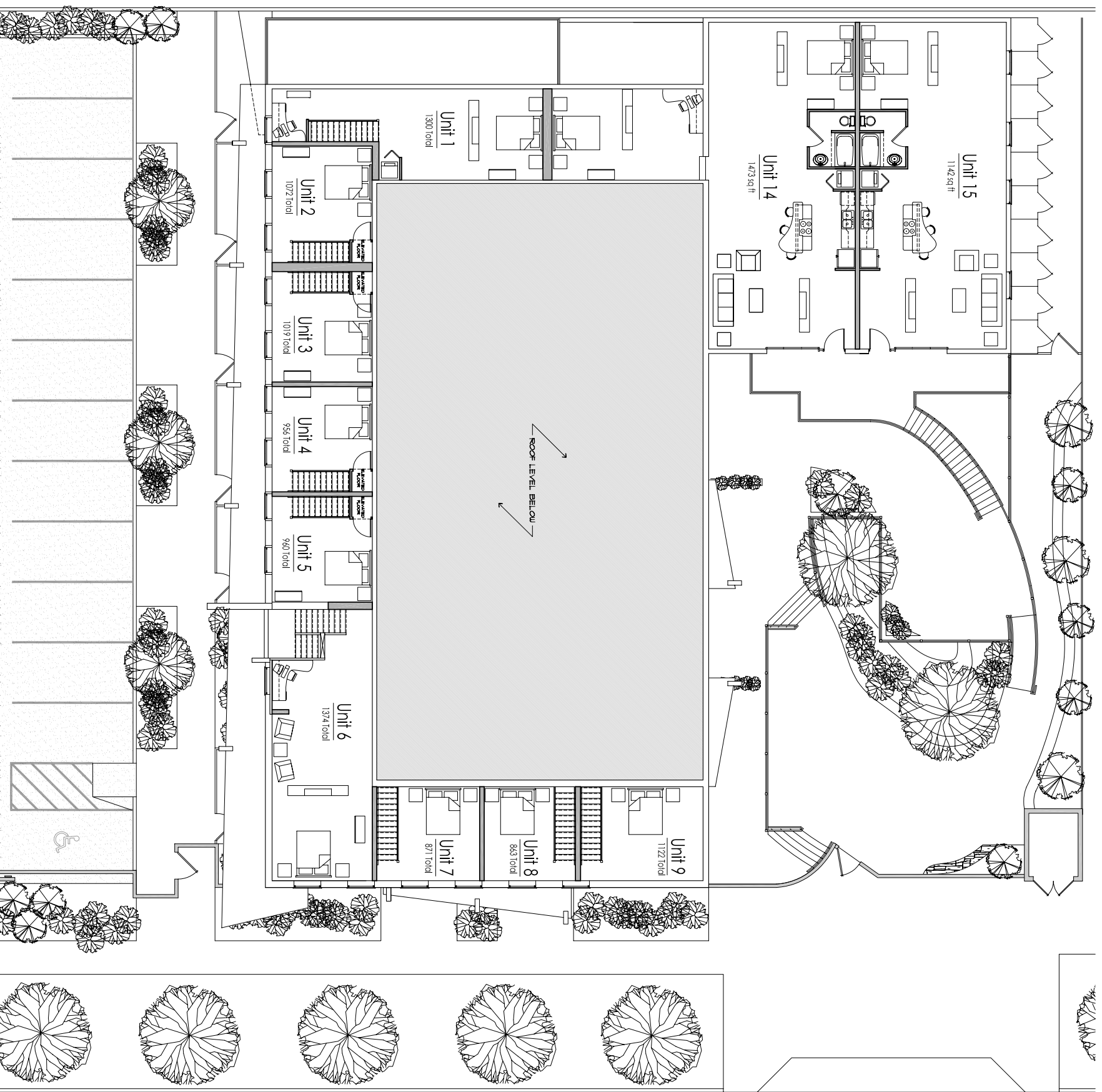
SECOND LEVEL FLOOR PLAN SCALE: 0' 8" NORTH
